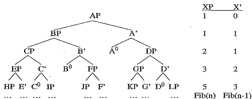
Figure 17.2. Maximal expansion of X-bar schema
