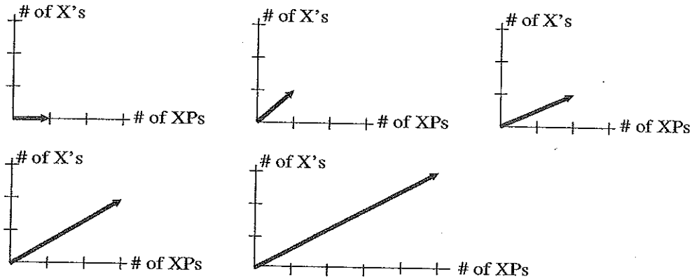
Figure 17.3. Vector representation of X-bar growth
