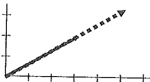
Figure 17.4. Eigenvector of the X-bar schema (solid line), and one step of growth (dashed line), corresponding to multiplication of the eigenvector by the X-bar matrix
