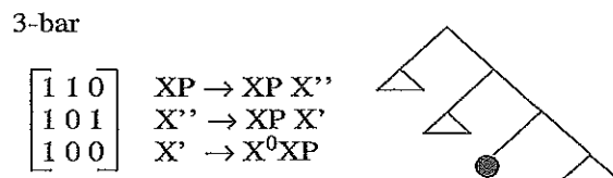
Figure 17.5. Matrix, rewrite rules, and tree schema for 3-bar, the Tribonacci grammar.
