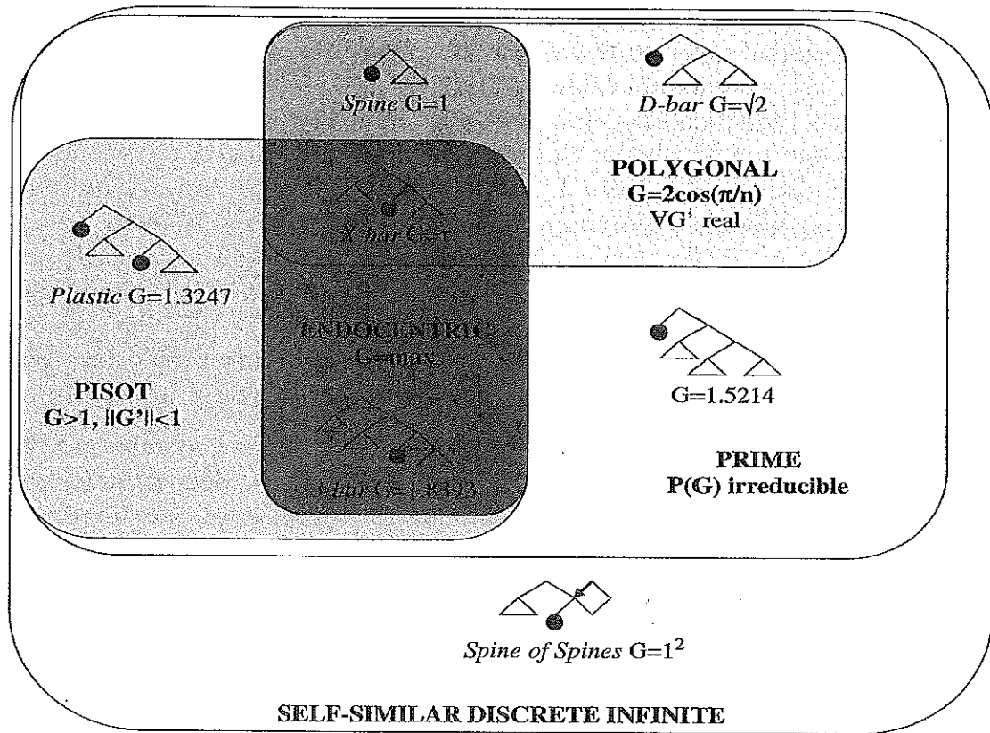
Figure 17.1. Intersection of spectral classes of phrasal recurrence patterns
