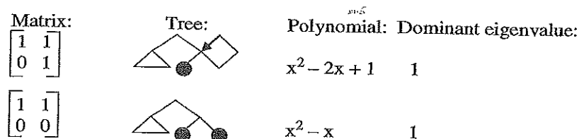
Figure 17.10. Composite systems of degree 2
