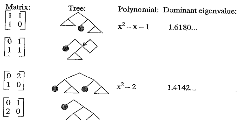
Figure 17.9. Prime systems of degree 2
